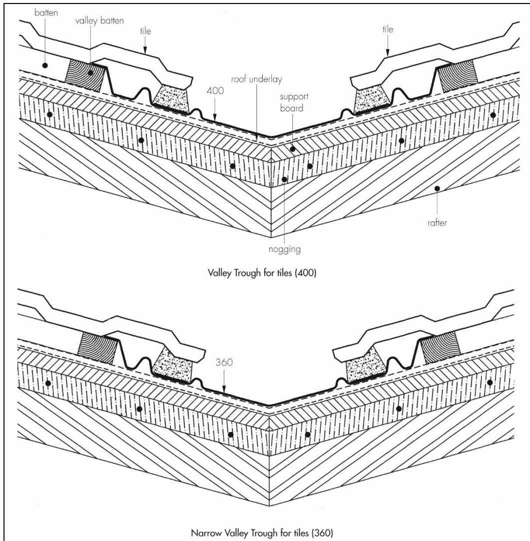
Figure 1 Klover GRP Valley Troughs for Tiles (400 and 360) - Batten Fix
